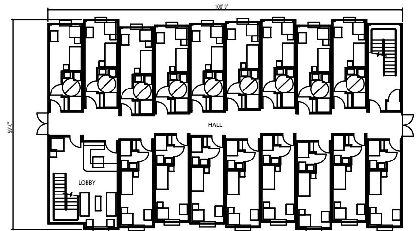
DORMITORY DESIGN
