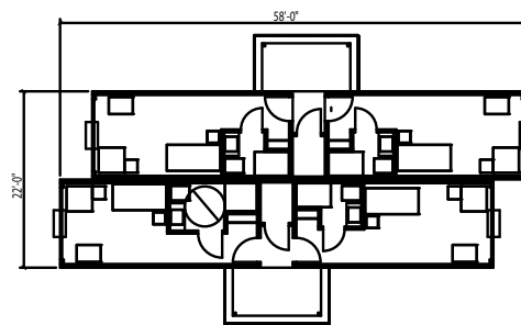
QUADPLEX DESIGN
