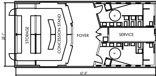
RESTROOM AND CONVENIENCE FACILITIES WITH BOLT-ON CONCESSION STAND, VERSION ONE "B"
