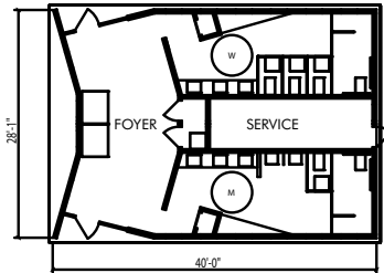
RESTROOM AND CONVENIENCE FACILITIES, VERSION ONE "A"
