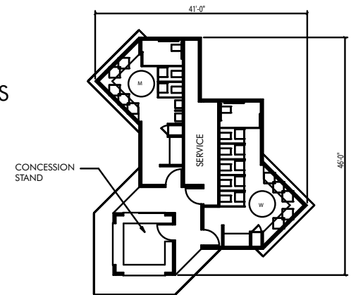
RESTROOM AND CONVENIENCE FACILITIES WITH BOLT-ON CONCESSION STAND, VERSION TWO
