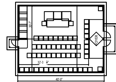
LARGE CLASSROOM / MEETING ROOM
